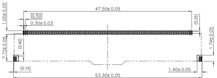
RECOMMENDED PCB PATTERN
